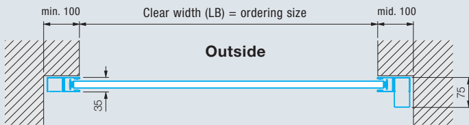
Fitting behind the opening
