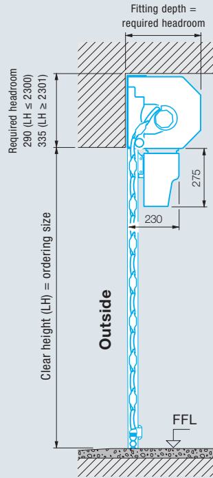
Fitting behind the opening
