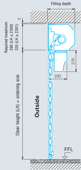
Fitting in the opening
